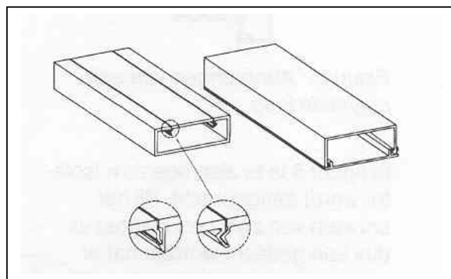
figuur 10: klikverbinding.
